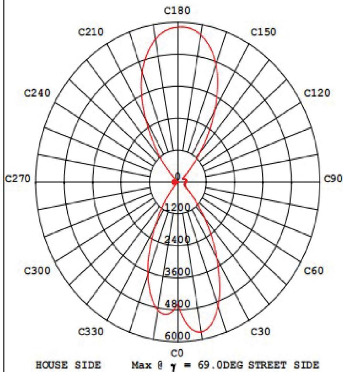
MAX INTENSITY CONE SURFACE DISTRIBUTION DIAGRAM
